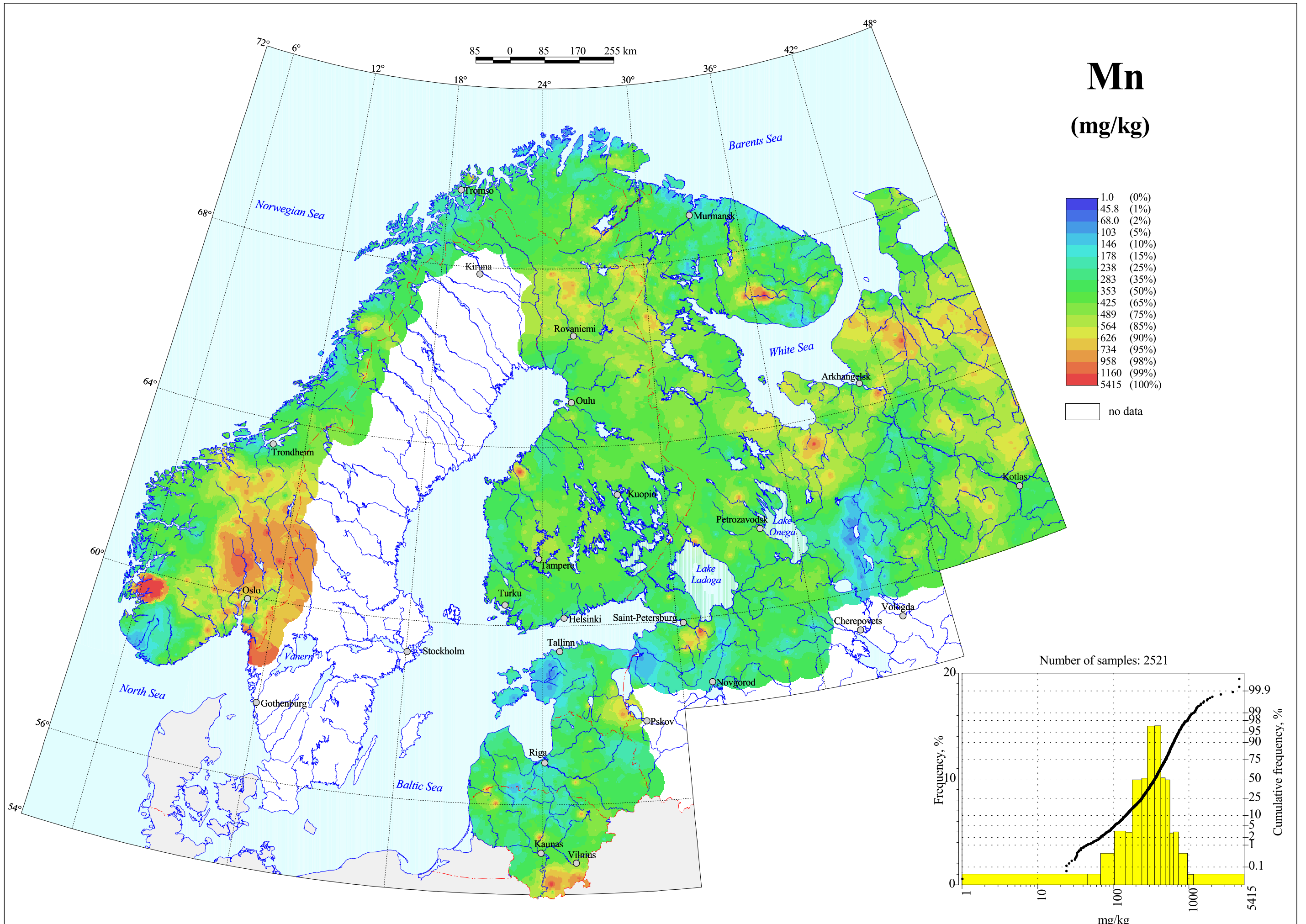
Manganese in Terrestrial Moss, Total Content
